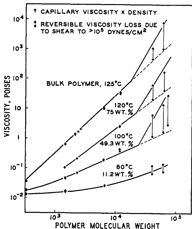
Figure 10.—Shear dependence of viscosity for polyisobutylenes in cetane.
