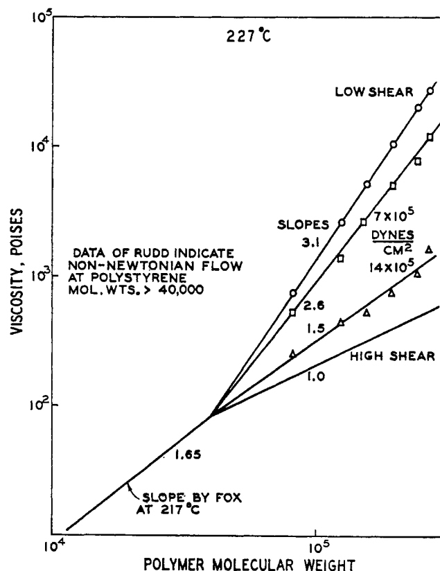
Figure 9.—Shear viscosities for polystyrene.
